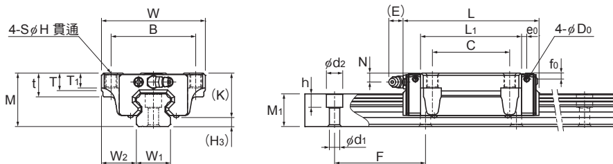
HSR15~35C/LC/CM/LCM型
