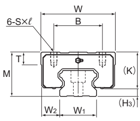
HSR100~150HR型
